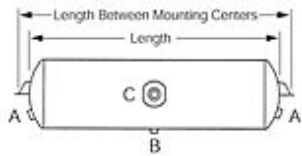
Type 3 - Flange Mounted
