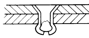
Countersunk
