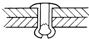
Dome Head
