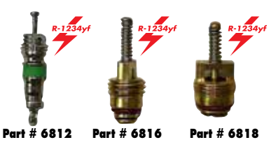
R-12, R-134a, R-1234yf Valve Cores Page 41
