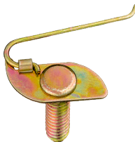
2818 (GM: 4689929, 4778814) Moulding Fastener Bolt: #10-24 x 3/4" Plate Length: 3/4" Plate Width: 5/16"
