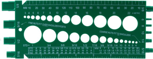
U.S.S., S.A.E. & Metric Bolt and Nut Gauge
